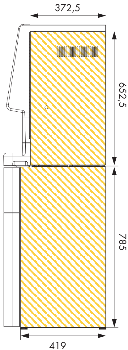
fianco destro right side
